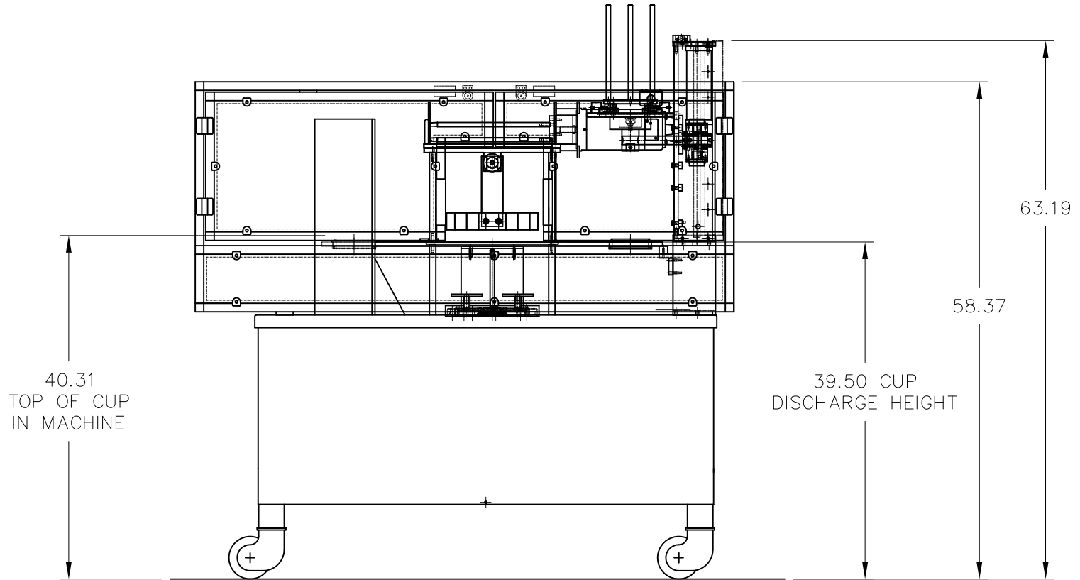
ELEVATION FROM OFF-END SIDE
