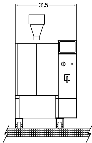
Viewed Facing Bagger (Operator's Side)
