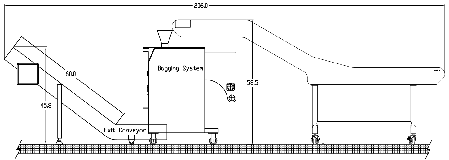
Viewed from right side of bagger
